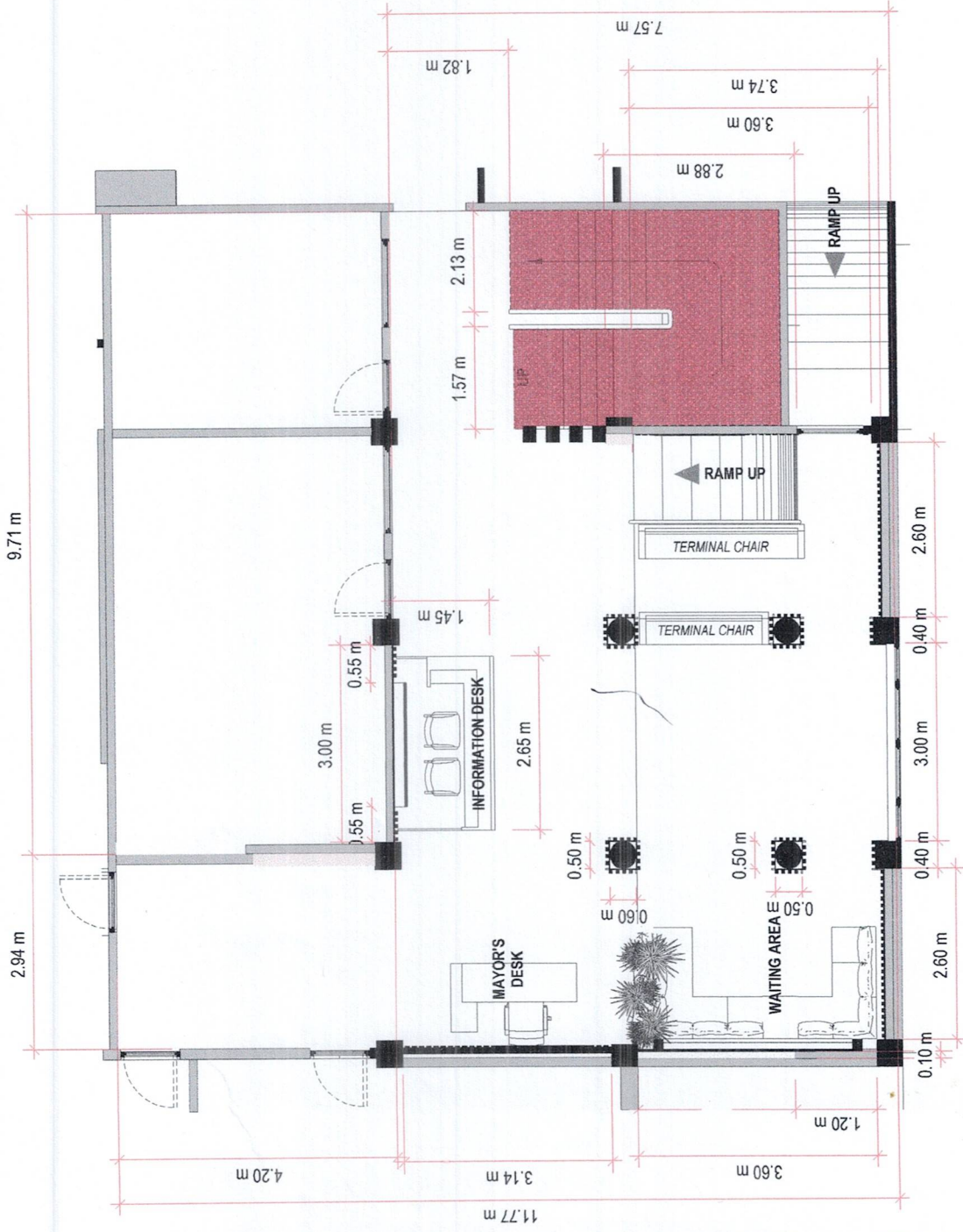
FLOOR PLAN SCALE: 1:100 MTS
