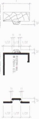
DETAIL OF JOINTS IN RIGID PAVEMENT SCALE: NTS
