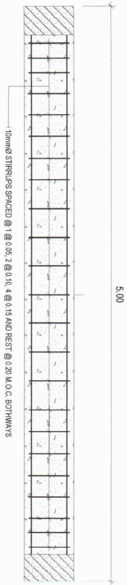
DETAIL OF BEAM SCALE 1:20 M
