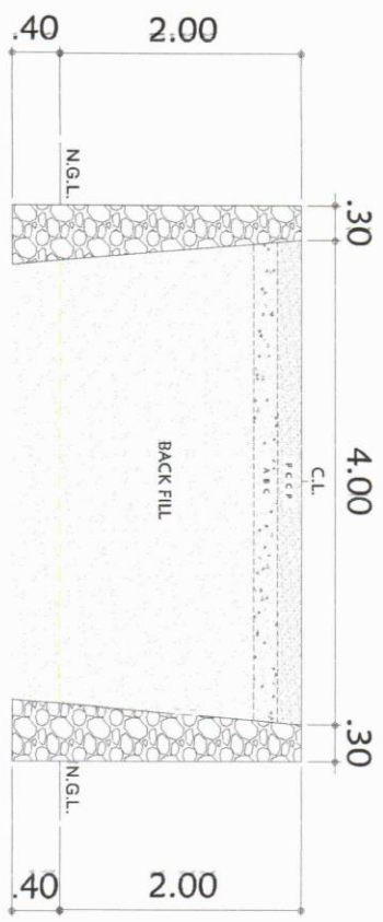
CROSS SECTION "A"
